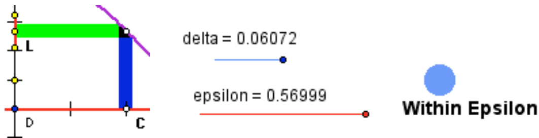
Figure 1. Epsilon-Delta Sliders
